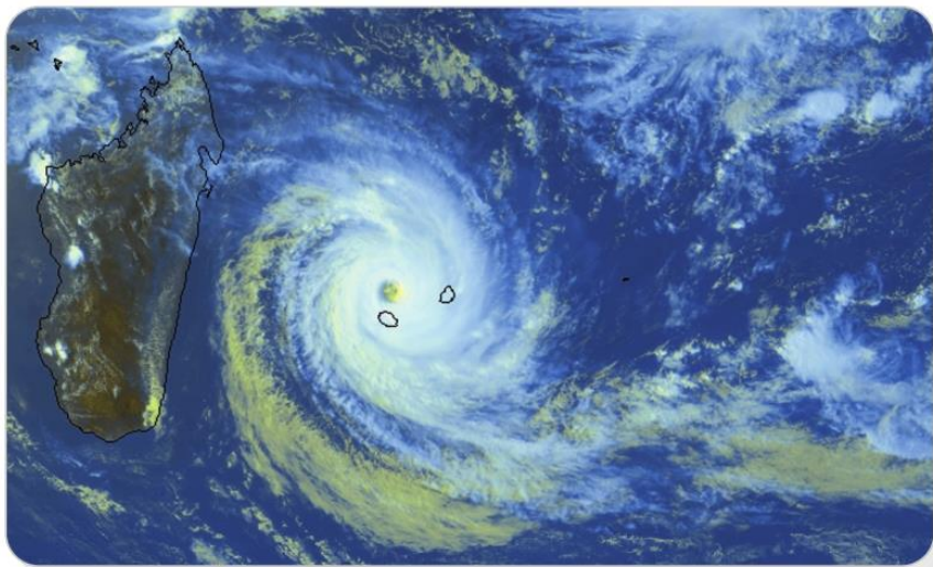
Image satellite du cyclone Dina (2002) - www.meteofrance.fr
